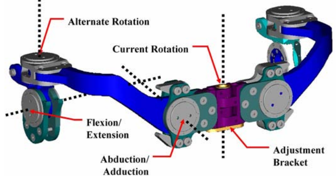
Fig. 3 BLEEX Hip Degrees of Freedom (viewed from back). Although both the abduction/adduction and flexion/extension axes pass through the center of the human hip joint, the rotation axis does not. The adjustment bracket, between the two abduction/adduction axes, is replaceable to accommodate wearers of various widths.
