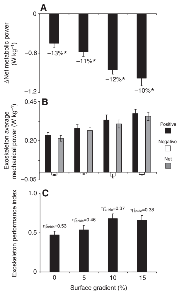
Fig. 4. Exoskeleton performance. Bar graphs show the mean (A) change in net metabolic power (powered–unpowered; W\text{kg}^{-1} ) as a result of powered assistance from bilateral ankle exoskeletons, (B) exoskeleton average positive (black), negative (white) and net (dark gray) mechanical power ( W\text{kg}^{-1} ) over a stride for powered walking and (C) exoskeleton performance index (unitless) of the nine subjects. Performance index indicates the fraction of ankle muscle–tendon positive work performed by plantar flexor muscle shortening rather than Achilles’ tendon recoil (i.e. muscle work fraction). Numbers above bars are equivalent ankle muscle–tendon ‘apparent efficiency’ values (see Materials and methods for details). For all panels, surface inclines increase from left (0%-level) to right (15%-uphill). Error bars are \pm 1 s.e.m. Asterisks (in A) indicate statistical significance for comparison of powered versus unpowered net metabolic power ( P < 0.05 ).
